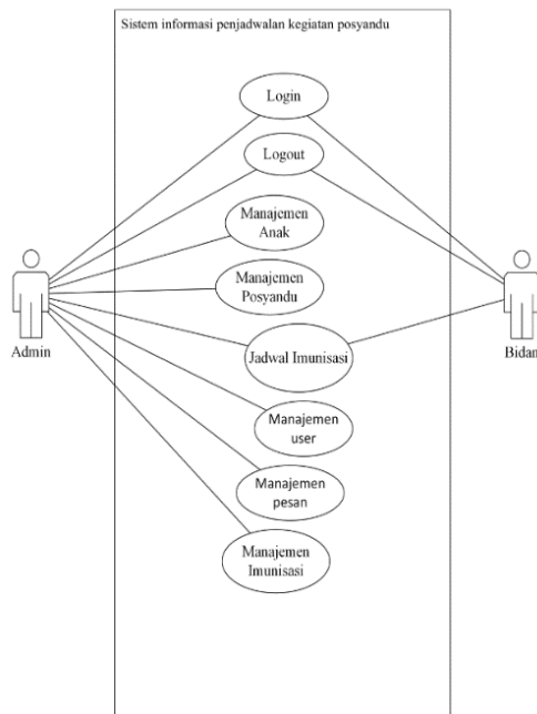
Gambar 2. Usecase Diagram
