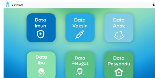
Gambar 4. Dashboard
